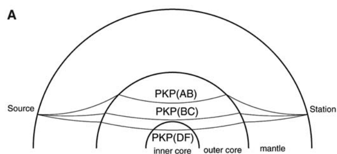
Fig. 1. Ray paths of PKP waves and example of waveform doublet used to detect temporal change of travel times through the inner core. (A) Ray paths of three branches of PKP waves turning in the solid inner core ( DF ), the bottom of the fluid outer core ( BC ), and the mid-outer core ( AB ). (B) Highly similar waveforms recorded at one station in Alaska. This waveform doublet 93 and 03 is the best recorded doublet of this study. m_b , body wave magnitude. (C) Superimposed and enlarged PKP waveforms from the box in (B), showing a misalignment of PKP(DF) . The waveforms are aligned on PKP(BC) and filtered from 0.5 to 1.0 Hz.
