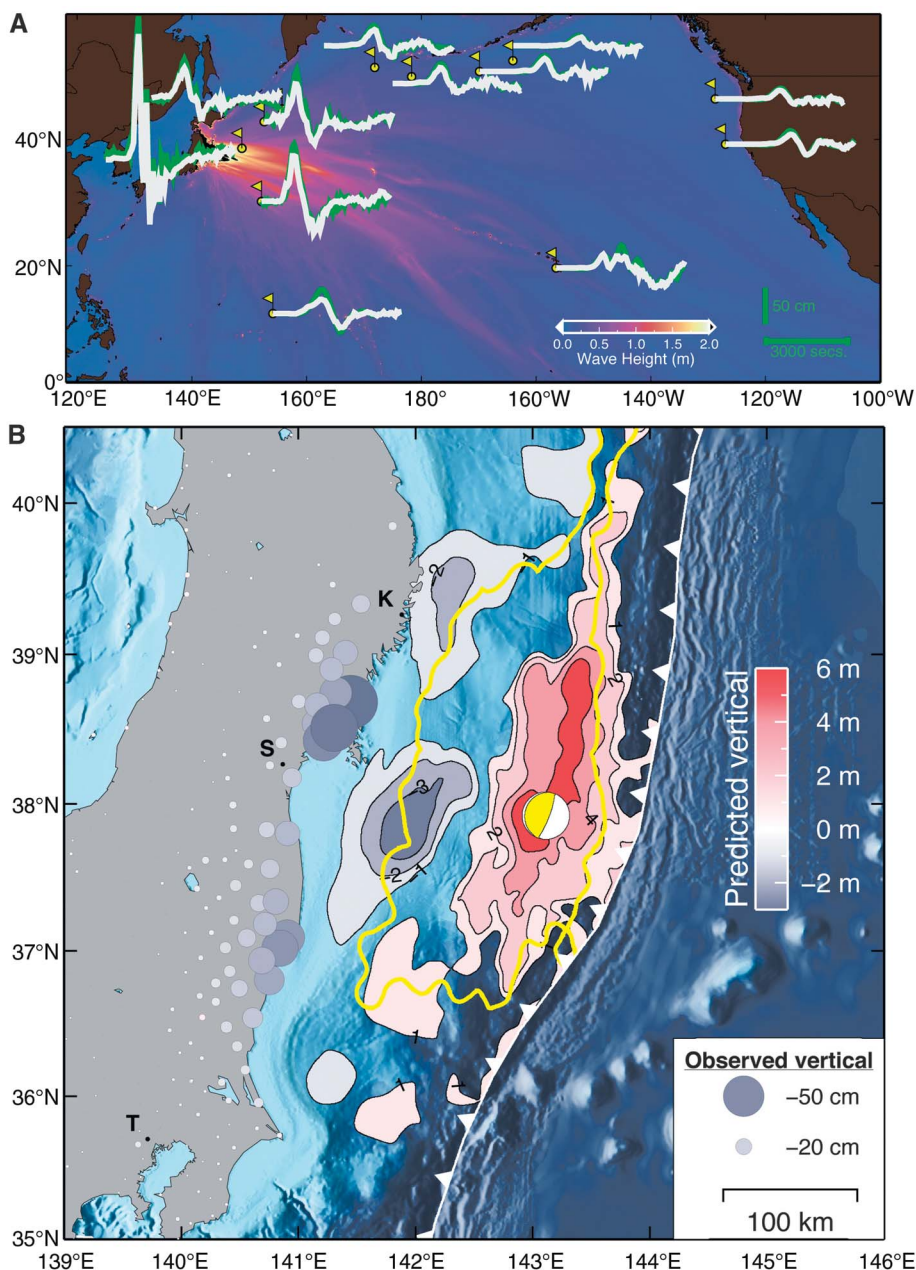
Fig. 2. (A) Observed (green) and predicted (white) deep ocean tsunami records of the Tohoku-Oki earthquake. The predicted records correspond to a model constructed using the mean of each fault slip parameter in the Bayesian inversion. These waveforms are superimposed on the map of maximum model-predicted tsunami height. (B) GPS vertical coseismic surface displacements (circles colored and scaled with amplitude) as well as model-predicted vertical sea-floor displacements (filled contours). Other overlay features are as in Fig. 1.
